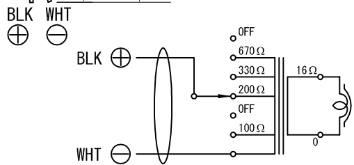
Wiring diagram
