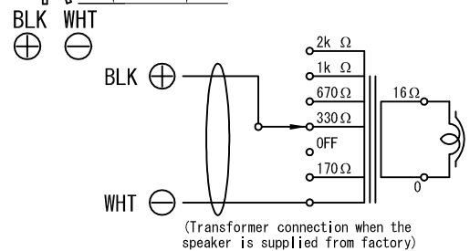
Wiring diagram
