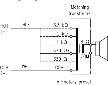
Wiring Diagram for PC-668R:
