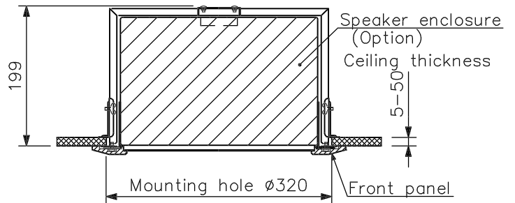
Ceiling Mounting
