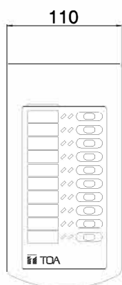
TOP View
