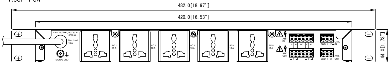
Front View
