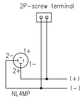
Wiring Diagram
