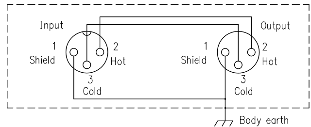
Circuit diagram
