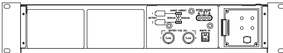
DS-029B without the front panel
